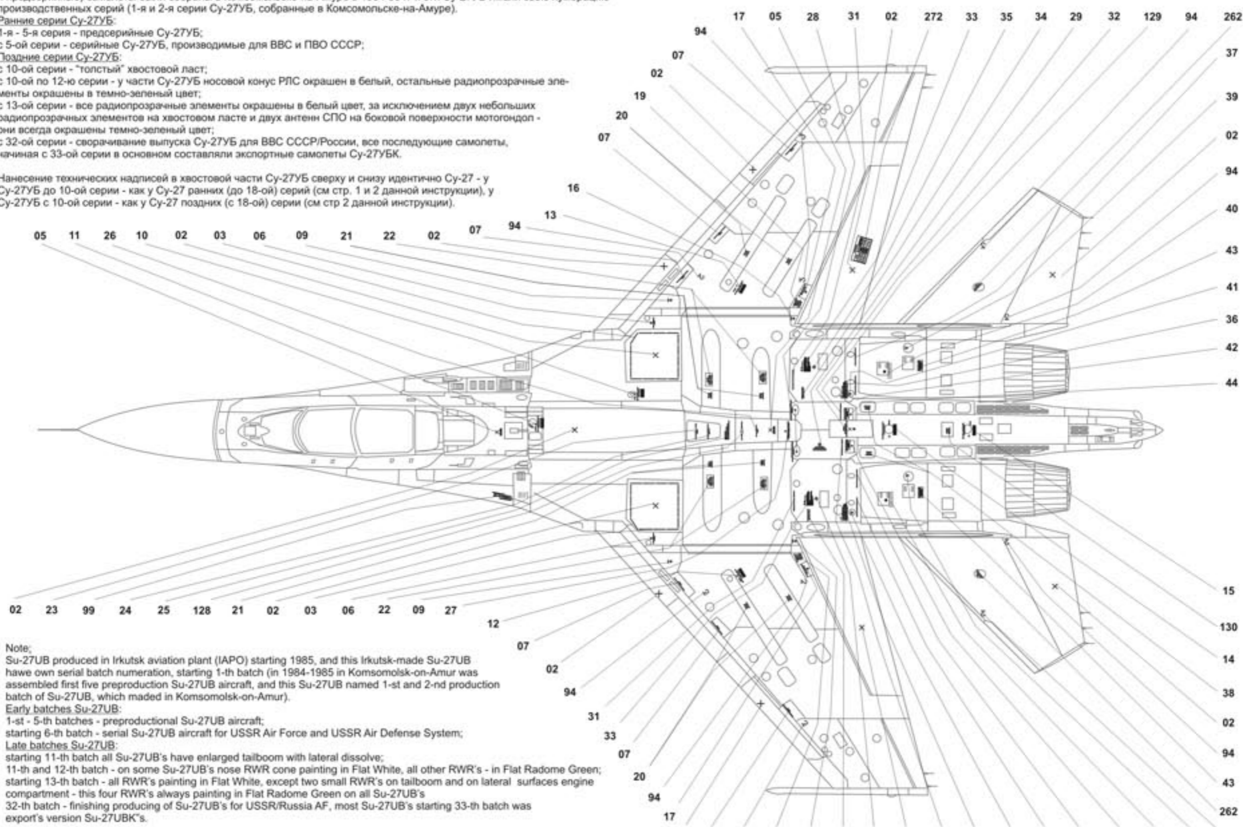
Su-27UB from late, after 10-th productional batch, top view
