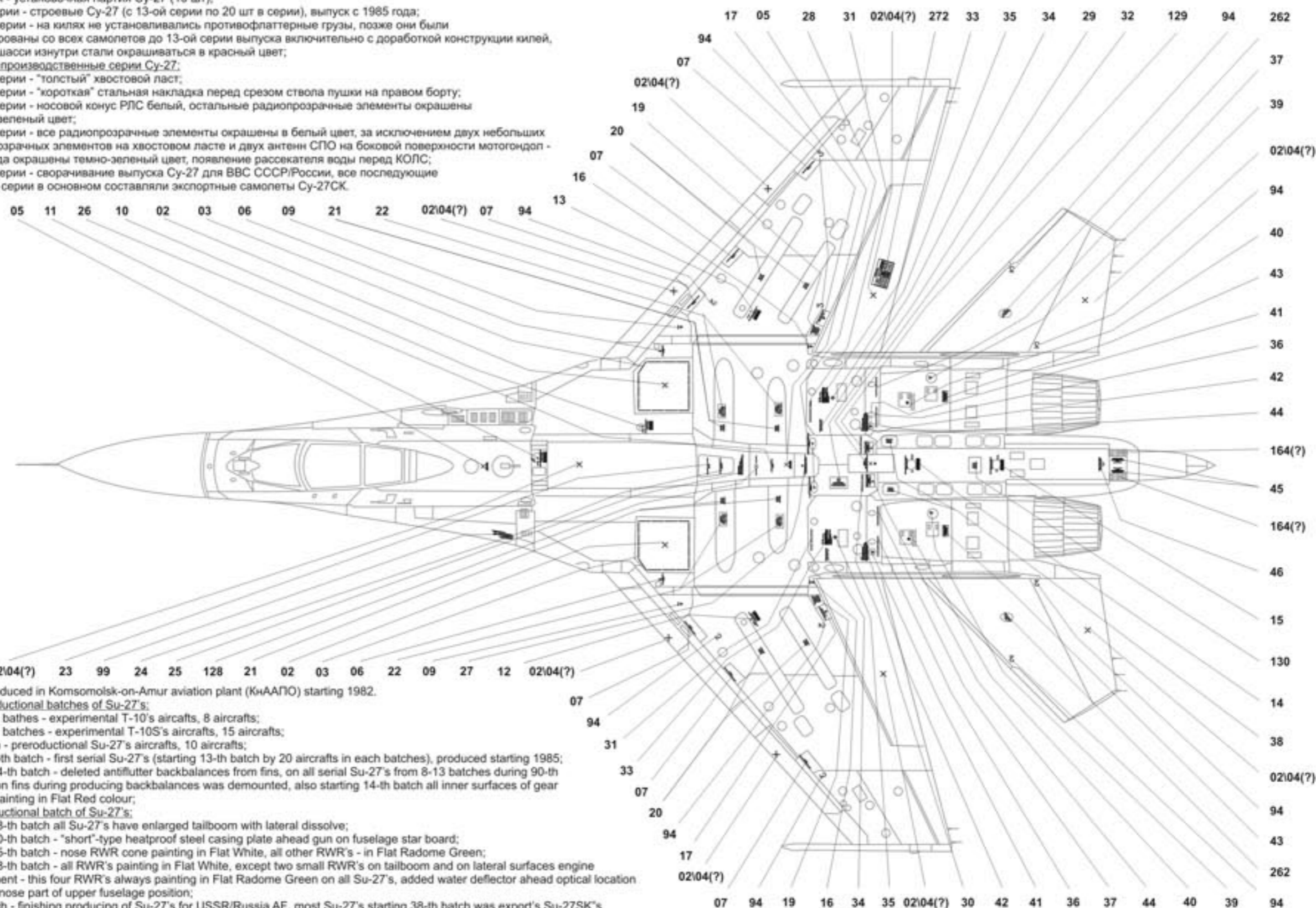
Su-27 from early, before 18-th, production batch, top view
